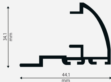
Enganche EMF8166
